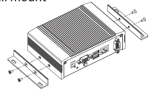
Wall mount
