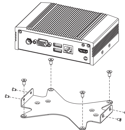
VESA mount
