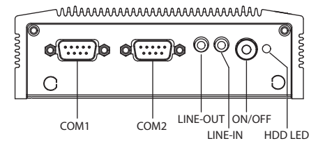
Rear Panel External I/O Mechanical Layout/Drawing
