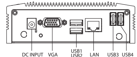
Rear Panel External I/O Mechanical Layout/Drawing
